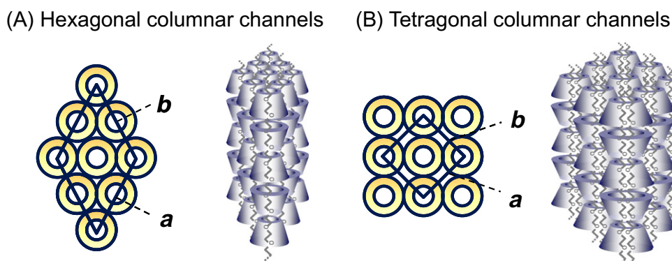
Figure 4. Schematic representation of crystal packing structures of \alpha -CyD (A) and \gamma -CyD (B) PPRXs.
