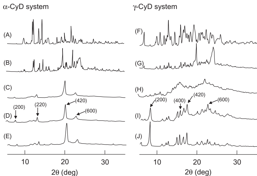
Figure 3. Powder X-ray diffraction patterns of PEG- \alpha -CDE/CyD PPRX. (A) \alpha -CyD alone, (B) PEG- \alpha -CDE/ \alpha -CyD physical mixture, (C) PEG- \alpha -CDE/ \alpha -CyD PPRX, (D) PEG- \alpha -CDE/pDNA/ \alpha -CyD PPRX, (E) PEG/ \alpha -CyD PPRX, (F) \gamma -CyD alone, (G) PEG- \alpha -CDE/ \gamma -CyD physical mixture, (H) PEG- \alpha -CDE/ \gamma -CyD PPRX, (I) PEG- \alpha -CDE/pDNA/ \gamma -CyD PPRX, (J) PEG/ \gamma -CyD PPRX.
