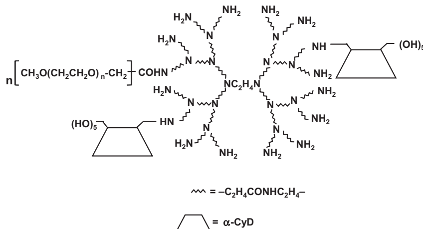
Figure 1. Chemical structure of PEG- \alpha -CDE.
